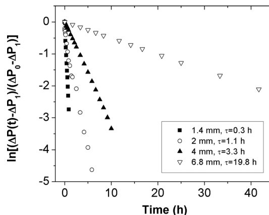
Fig. 9 Natural log plot of unaccomplished change in the difference in pressure across the diaphragm for different radii. The pressure differences are: instantaneous, \Delta P(t) ; initial, \Delta P_0 ; and final \Delta P_1 . Slopes of the linear regressions were used to estimate time constants of equilibration, \tau , indicated in the legend (slope = -\tau^{-1} ).
