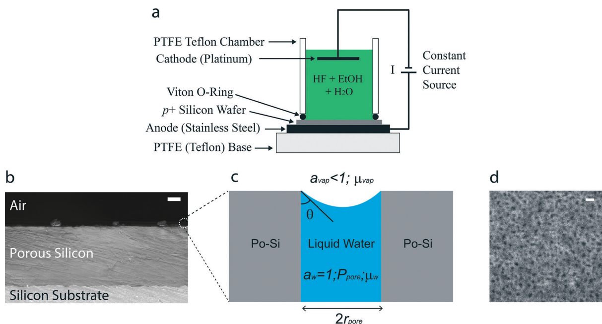
Fig. 4 Nanoporous silicon membrane. (a) Electrochemical etch cell (cross-section) used for the formation of porous silicon. (b) Scanning electron micrograph cross-section of porous silicon membrane; scale bar = 1 \mu\text{m} . (c) Schematic of an individual pore cross-section within the porous silicon membrane showing the liquid–vapor interface, the contact angle of water with the membrane wall ( \theta ), and pore radius ( r_{\text{pore}} ). (d) Nanoporous silicon (grey), top view, showing surface pores (dark spots) with diameters ( 2r_{\text{pore}} ) ranging from 1–5 nm; scale bar = 10 \text{ nm} .
