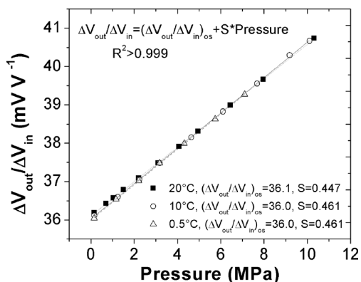
Fig. 7 Reproducibility and temperature-dependence of pressure sensor calibrations of a 1 mm radius diaphragm device at 20 °C, 10 °C, and 0.5 °C. ( \Delta V_{\text{out}}/\Delta V_{\text{in,os}} [ \text{mV V}^{-1} ] is the voltage offset at \Delta P = 0 MPa pressure, and S [ \text{mV V}^{-1} \text{MPa}^{-1} ] is the sensitivity.
