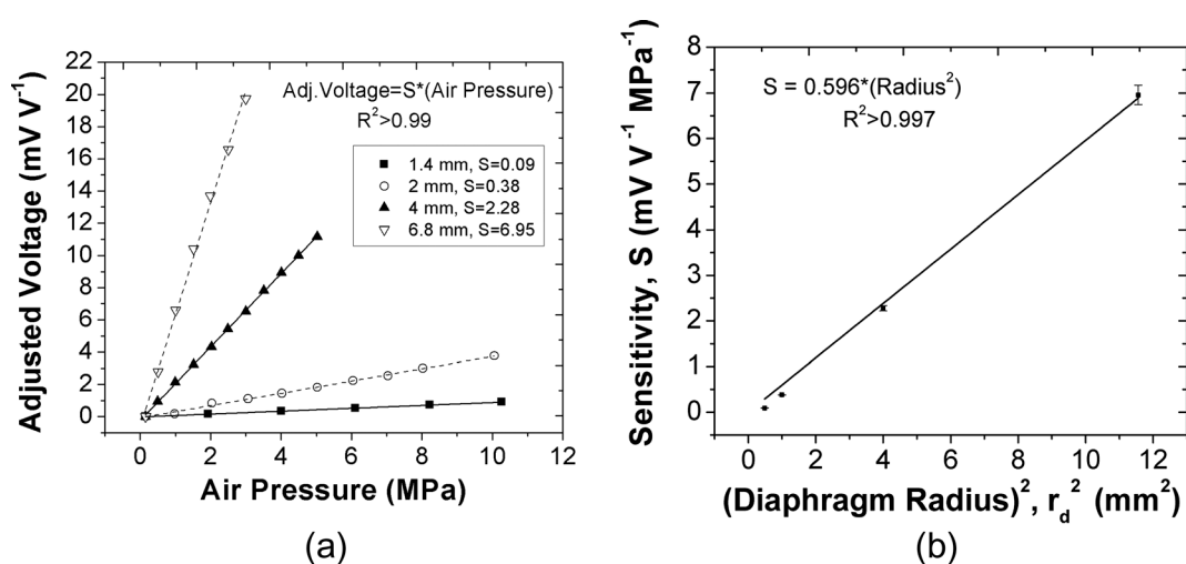
Fig. 6 Pressure sensor calibration: (a) microtensimeter calibrations using positive pressures of air for diaphragms of different radii. The responses plotted were shifted by their offsets ( (\Delta V_{\text{out}}/\Delta V_{\text{in}}) - (\Delta V_{\text{out}}/\Delta V_{\text{in}})_{\text{os}} ; eqn (7)). Legend: for each diaphragm radius in mm, the slope of the linear regressions represent the sensitivity, S [ \text{mV V}^{-1} \text{ MPa}^{-1} ] (eqn (7) and (8)). Offset voltages were: 28.5 \text{ mV V}^{-1} (0.7 mm), 27.3 \text{ mV V}^{-1} (1 mm), 3.8 \text{ mV V}^{-1} (2 mm), and 27.5 \text{ mV V}^{-1} (3.4 mm). Higher values of 'S' indicate greater sensitivity to pressure. (b) Sensitivity versus (diaphragm radius) 2 = r_d^2 (see eqn (7) and (8)) for calibrations in (a).
