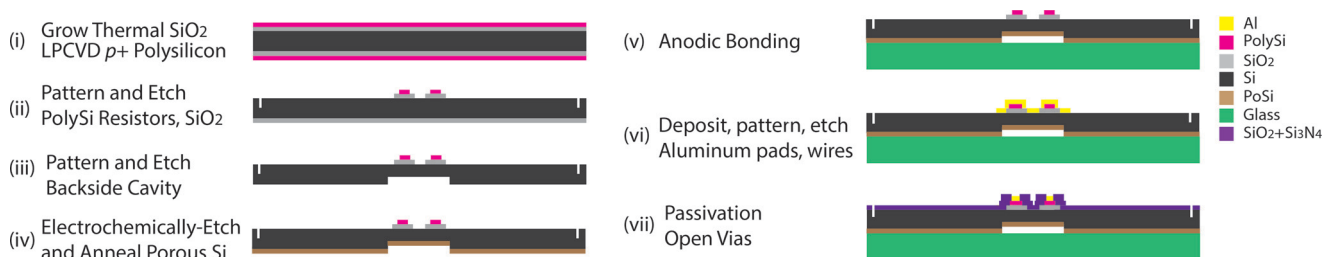
Fig. 3 Microtensiometer fabrication process flow (abridged). Detailed process flow provided in the ESI† Fig. S1.
