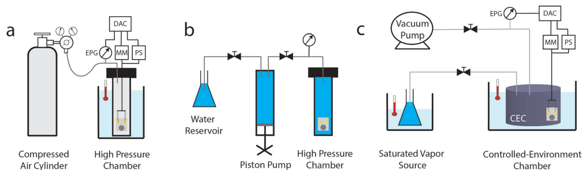
Fig. 5 Experimental setup for calibration, filling, and testing of the microtensiometer. (a) Positive pressure of air used to calibrate pressure sensor to P_{\text{air}} > 10 MPa at constant temperature. DAC = Data acquisition card + computer; MM = digital multimeter; PS = digital power supply; EPG = electronic pressure gauge. (b) Filling under high pressure ( P_{\text{liq}} > 5 MPa) of water. (c) Controlled environment chamber (CEC; dark grey air-tight cylinder) used to equilibrate sensor with sub-saturated vapor stream for testing.
