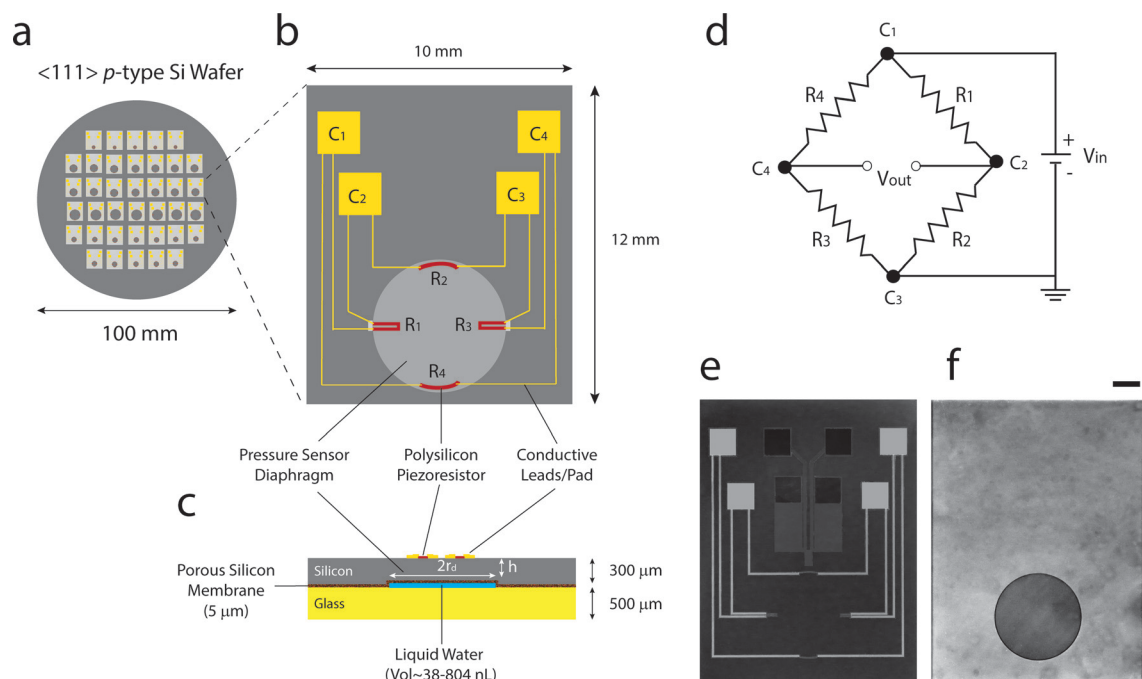
Fig. 1 Microtensiometer. (a) Organization of tensiometers on a 4" p-type \langle 111 \rangle silicon wafer. Wafer contains 38 sensors with diaphragms of various radii: 0.7 mm (5 copies), 1 mm (12 copies), 2 mm (14 copies), and 3.4 mm (7 copies). (b–c) Top (b) and cross-sectional (c) views of a sensor with a 2 mm-radius diaphragm. Aluminum leads and contact pads are shown in yellow and polysilicon resistors are shown in red. In (b), contact pads for Wheatstone bridge are labeled C_1 – C_4 and resistors are labeled R_1 – R_4 . In (c), the diaphragm radius and thickness are labeled r_d and h , respectively. (d) Wheatstone bridge configuration of piezoresistors and connections for applied ( V_{in} ) and measured ( V_{out} ) voltages. Labels of contact pads and resistors correspond to those in (b). (e) Photo showing top-view of an individual fabricated sensor (die) with 2 mm-radius diaphragm. Patterned oxide for a platinum resistance thermometer (PRT) is visible in the center, top of the die. No PRT was fabricated on the microtensiometers described in this paper. (f) Bottom-view of device shown in (e) showing the porous silicon membrane surface and circular cavity of depth \sim 25 \mu\text{m} . Scale bar = 1.5 mm.
