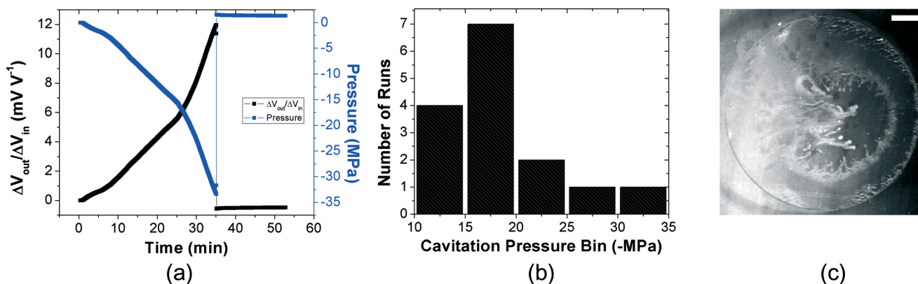
Fig. 8 Stability limit. (a) Transient response of a microtensimeter (1 mm radius diaphragm) exposed to ambient relative humidity ( a_w \sim 0.6 \equiv \Psi_w \cong -54 \text{ MPa} ). Voltage response ( \Delta V_{\text{out}}/\Delta V_{\text{in}} – black points and left axis) and pressure difference across diaphragm based on calibration (blue points and right axis) are shown. At 35 minutes, the liquid within the cavity cavitated and the pressure returned to a positive value. (b) Histogram of the stability limits of microtensimeters for 15 runs with 10 different sensors. (c) Snapshot of cavitation in the liquid cavity of a microtensimeter (3.4 mm radius diaphragm). Cavitation image captured using a high-speed camera (MotionPro HS-3, Redlake Imaging, Cheshire, CT) at 3000 fps through the glass wafer. See ESI.† Scale bar = 1 mm.
