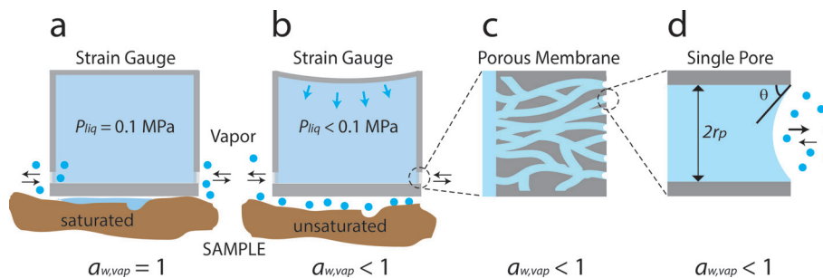
Fig. 2 Concept of tensiometry. (a) Bulk liquid in equilibrium ( P_{\text{liq}} = p_{\text{vap}} \cong 0.1 MPa) with a saturated vapor ( a_w = 1 ); tensiometer placed in a sample, e.g. saturated soil) through a porous membrane (shown in light grey on two lower sides of the cavity); liquid-vapor equilibrium exists and no net evaporation occurs from the bulk liquid. (b) Sub-saturated vapors ( a_{w,\text{vap}} < 1 ; tensiometer placed in unsaturated soil as an example) lower the hydrostatic pressure in the bulk liquid ( P_{\text{liq}} < 0.1 MPa) by driving evaporative loss of water from the membrane. Changes in hydrostatic pressure are measured by measuring the deflection of a flexible diaphragm (strain gauge shown as curved plate on top side of cavity). (c) Porous membrane at the interface of the cavity couples external vapor with bulk water inside the cavity. (d) Close-up of a single pore within the membrane showing a concave air-liquid interface pinned at the mouth of the pore; r_p is the pore radius and \theta is the contact angle of the liquid with the wall of the membrane.
