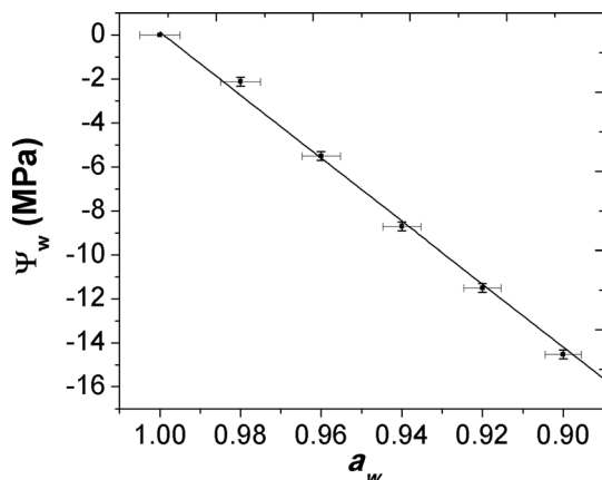
Fig. 10 Comparison to equation of state. Measured (filled squares) and IAPWS-95 calculated (line) water potentials ( \Psi_w , MPa) at various vapor activities ( a_w ) as defined by the vapor pressures in vacuum (Fig. 5c). Measurements were performed with a 1 mm radius diaphragm at 20 °C. Error bars on water potential are the uncertainties reported in Table 2 and those on activity are dominated by the propagation of the uncertainty in temperature through eqn (4).
